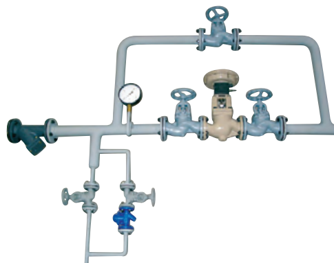
Steam dosing unit with electro-pneumatic valve DDU - complete piping
